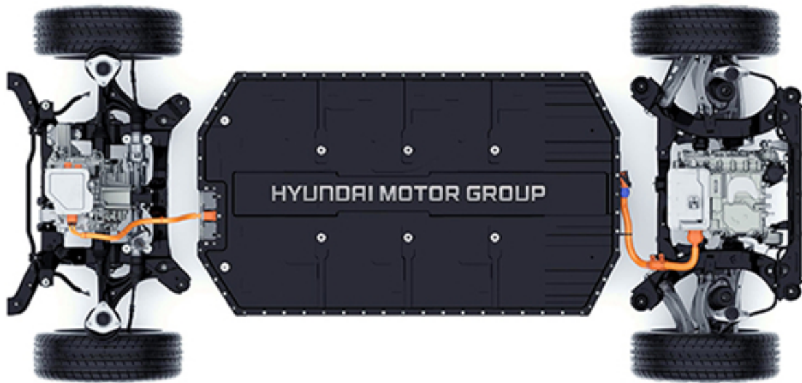
现代汽车集团纯电动汽车平台E-GMP ( Electric-Global Modular Platform )
